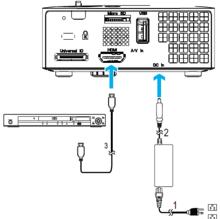
Connecting a DVD Player Using a HDMI Cable
