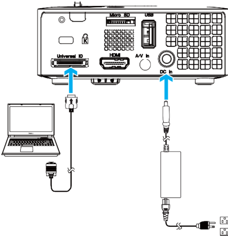
Connecting a Computer Using a VGA Cable
