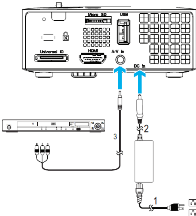
Connecting a DVD Player Using a A/V to RCA Cable
